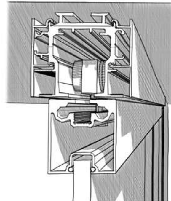
Asymmetrical folding sistem Five doors panel with perimetrical aluminium profile, three folding right and two left
