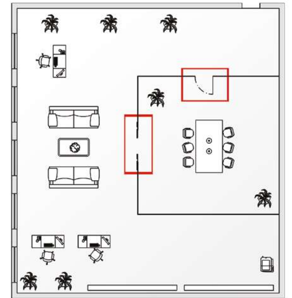
Sistema scorrevole | Sliding system
