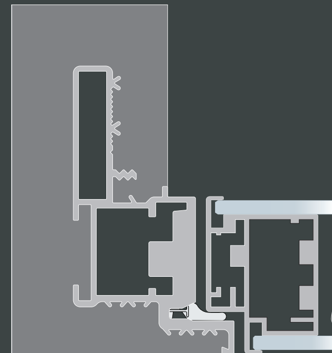
PORTA A SPINGERE PULL OPENING
