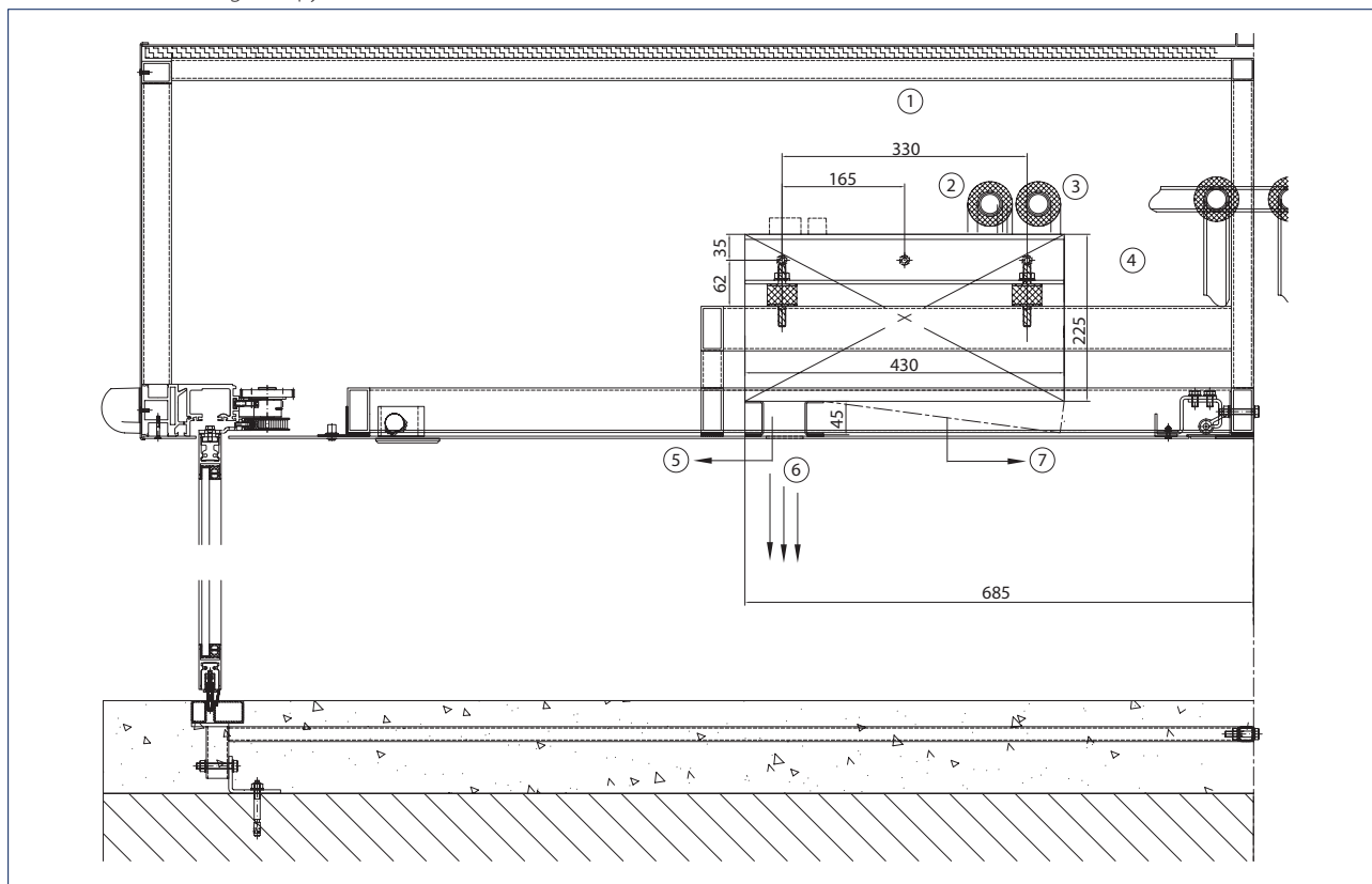
Hot-air curtain in ceiling canopy
