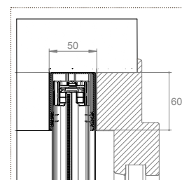
■ LINDAPLUS INCAS STANDARD
